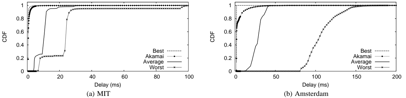
Figure 9: CDF of RTTs for Akamai paths for two PL nodes.
