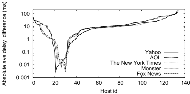
Figure 10: Latency gains for all measured PL nodes.
